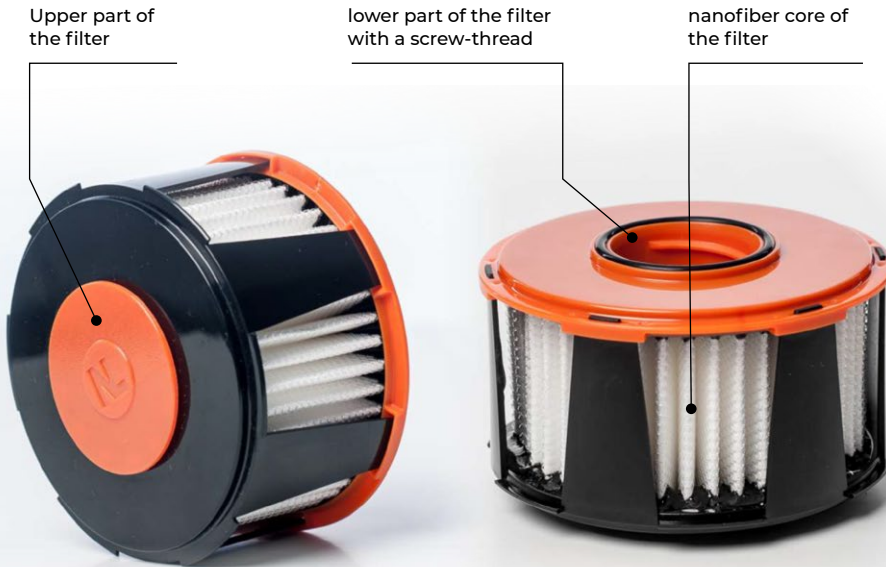
Nanofiber filter structure
